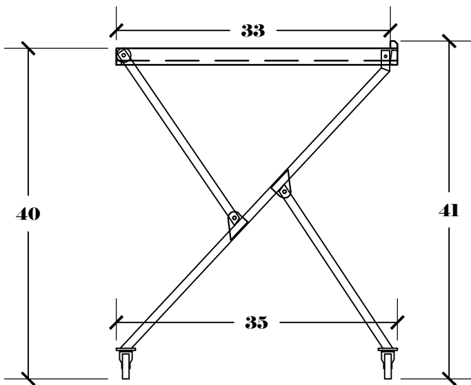
ASSEMBLY/UTILITY POSITION DIMS
