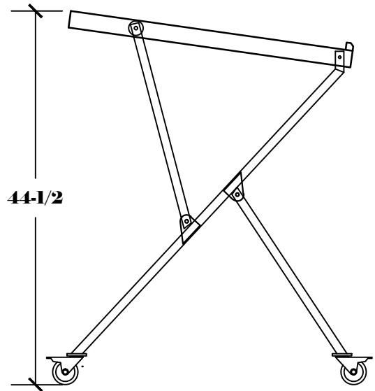
PLAN VIEWING/DETAILING POSITION DIMS
