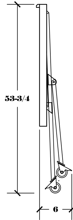
STORAGE/TRANSPORTATION POSITION DIMS
